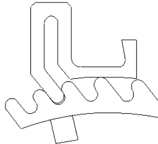
Instrumented Dynamometric Clip placed between the buckle and the ladder
