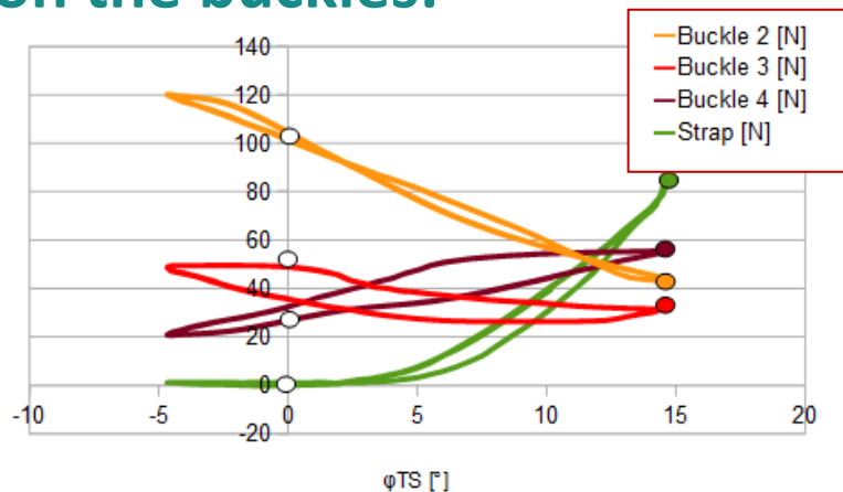
Load cycles on different buckles of the ski boot during cyclic FLEX testing
