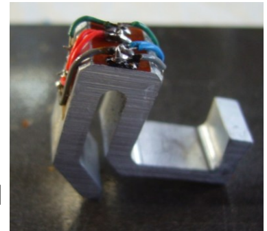
Instrumented Dynamometric Clip placed between the buckle and the ladder
