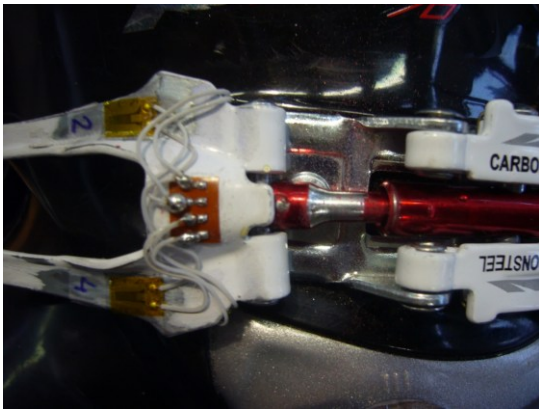
Sensors applied directly to the ski boot buckles
